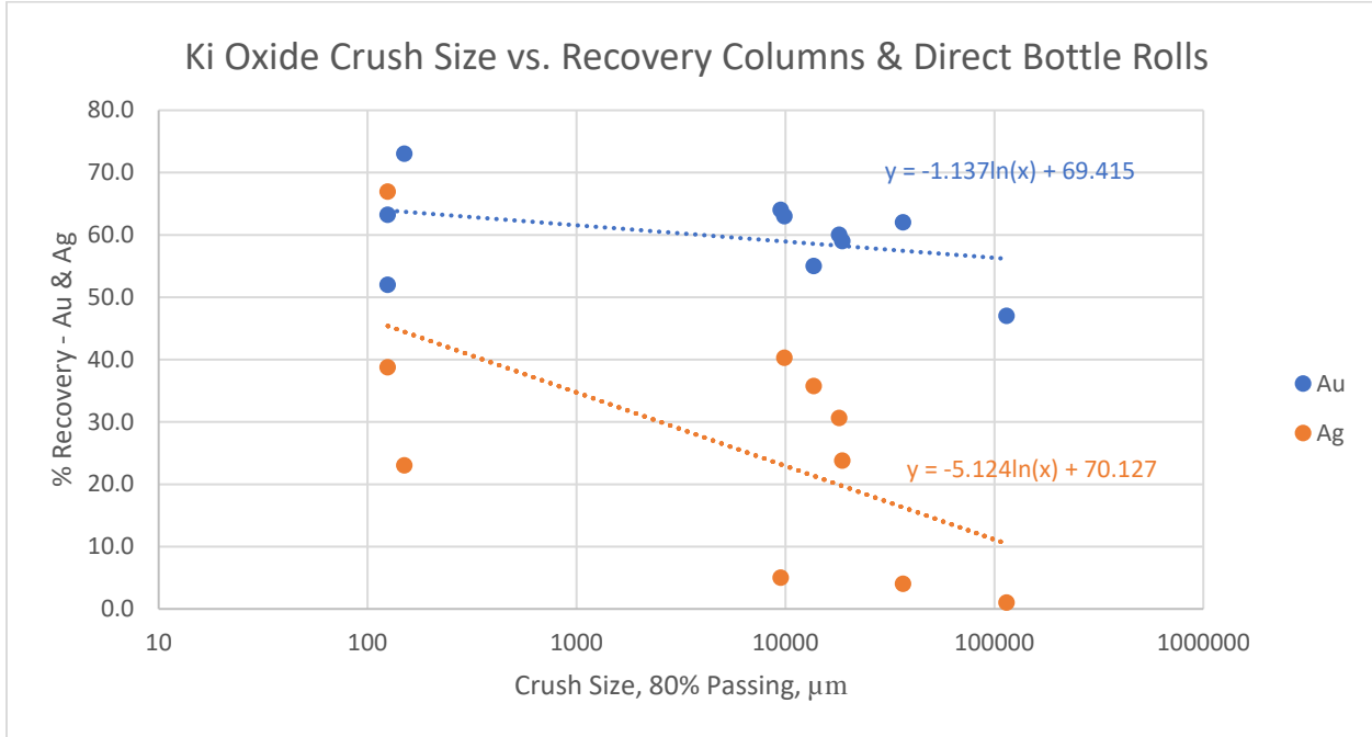
Figure 13.10 Ki Oxide Recovery vs. Crush Size
