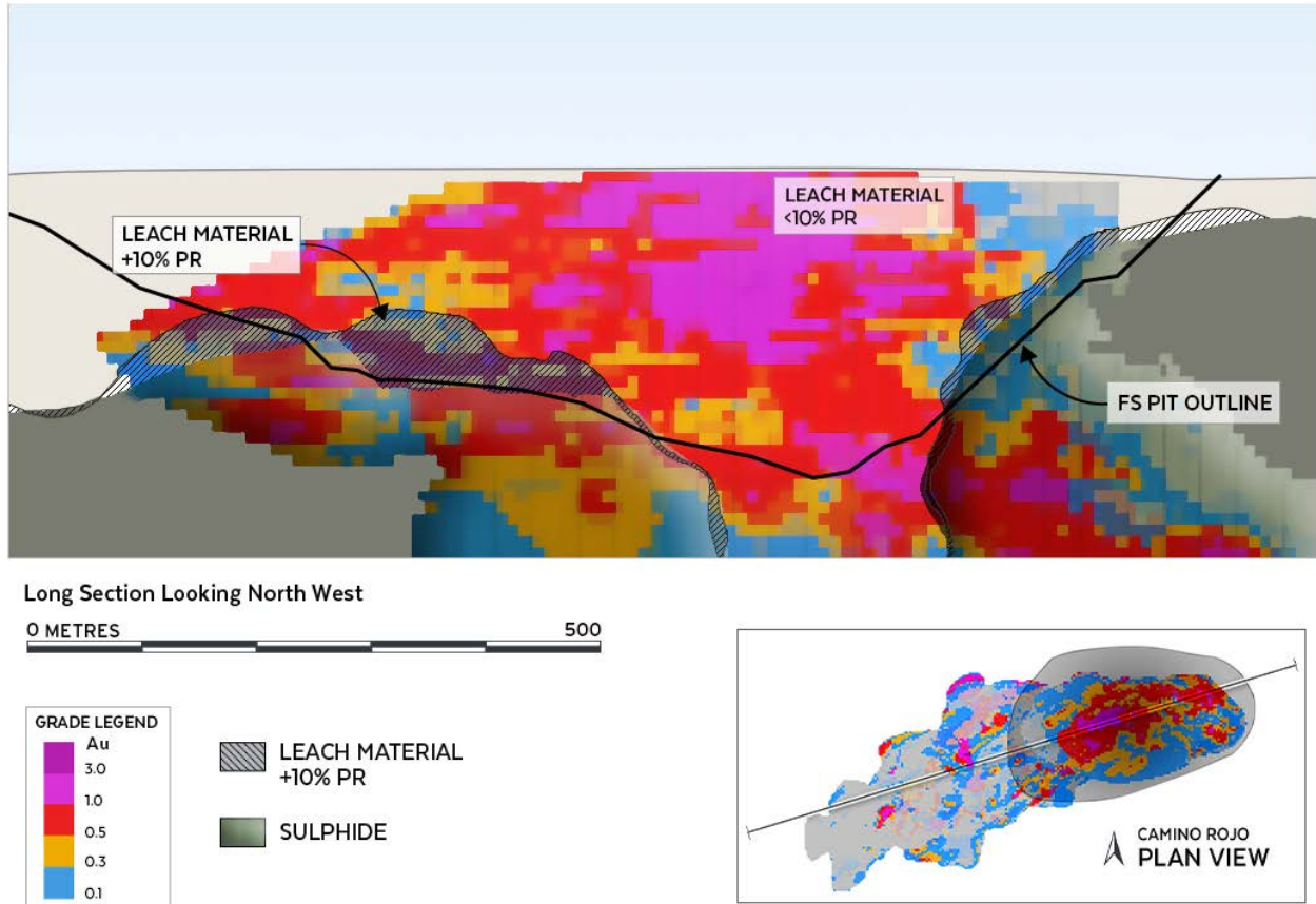
Figure 13.14 Areas with +10% Preg-Robbing Test Results
