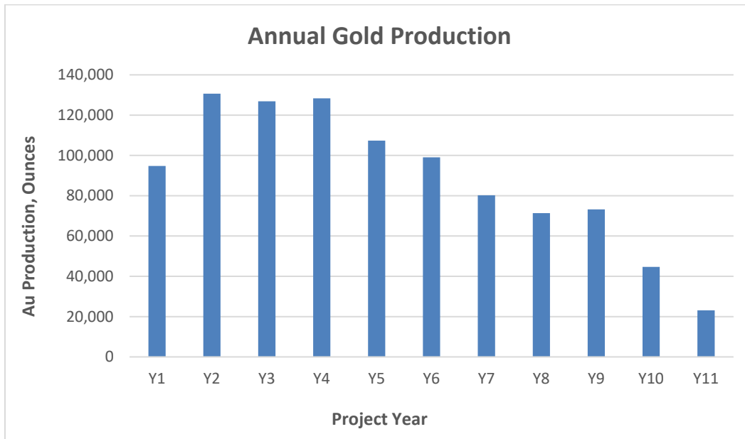
Figure 22.1 Annual Gold Production
