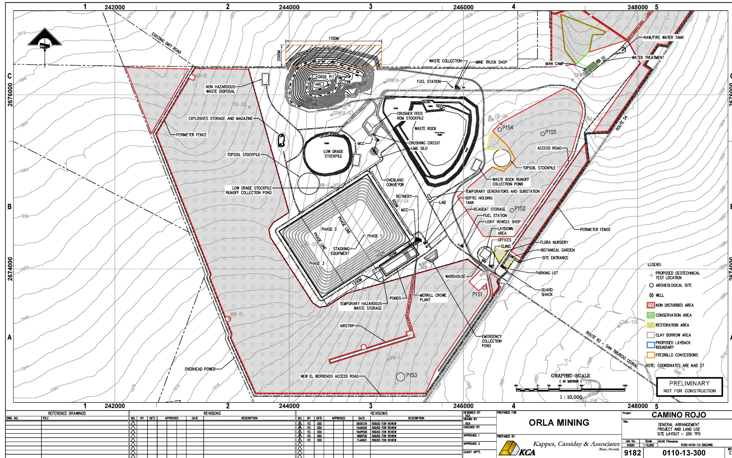
Figure 17.2 Project General Arrangement
