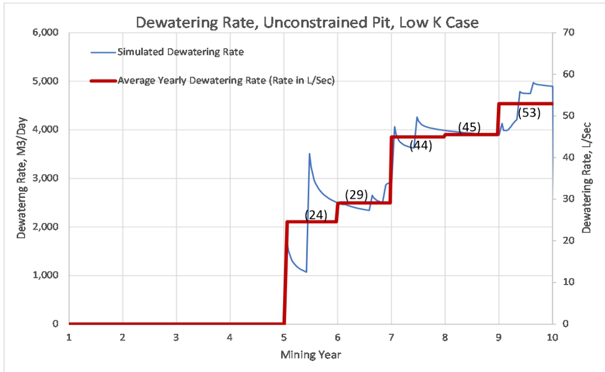
Figure 24.5 Simulation Dewatering Rates for Law and High K Scenarios, Camino Rojo Project, Zacatecas
