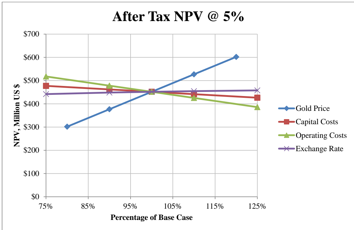
Figure 1.2 NPV @ 5% vs. Gold Price, Capital Cost, Operating Cost & Exchange Rate
