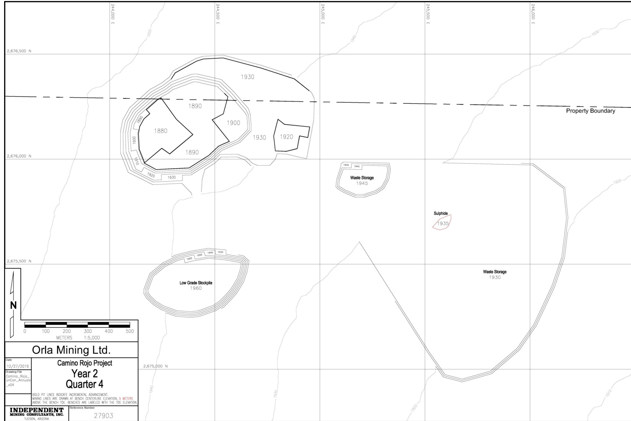
Figure 16.7 End of Year 2, IMC 2019
