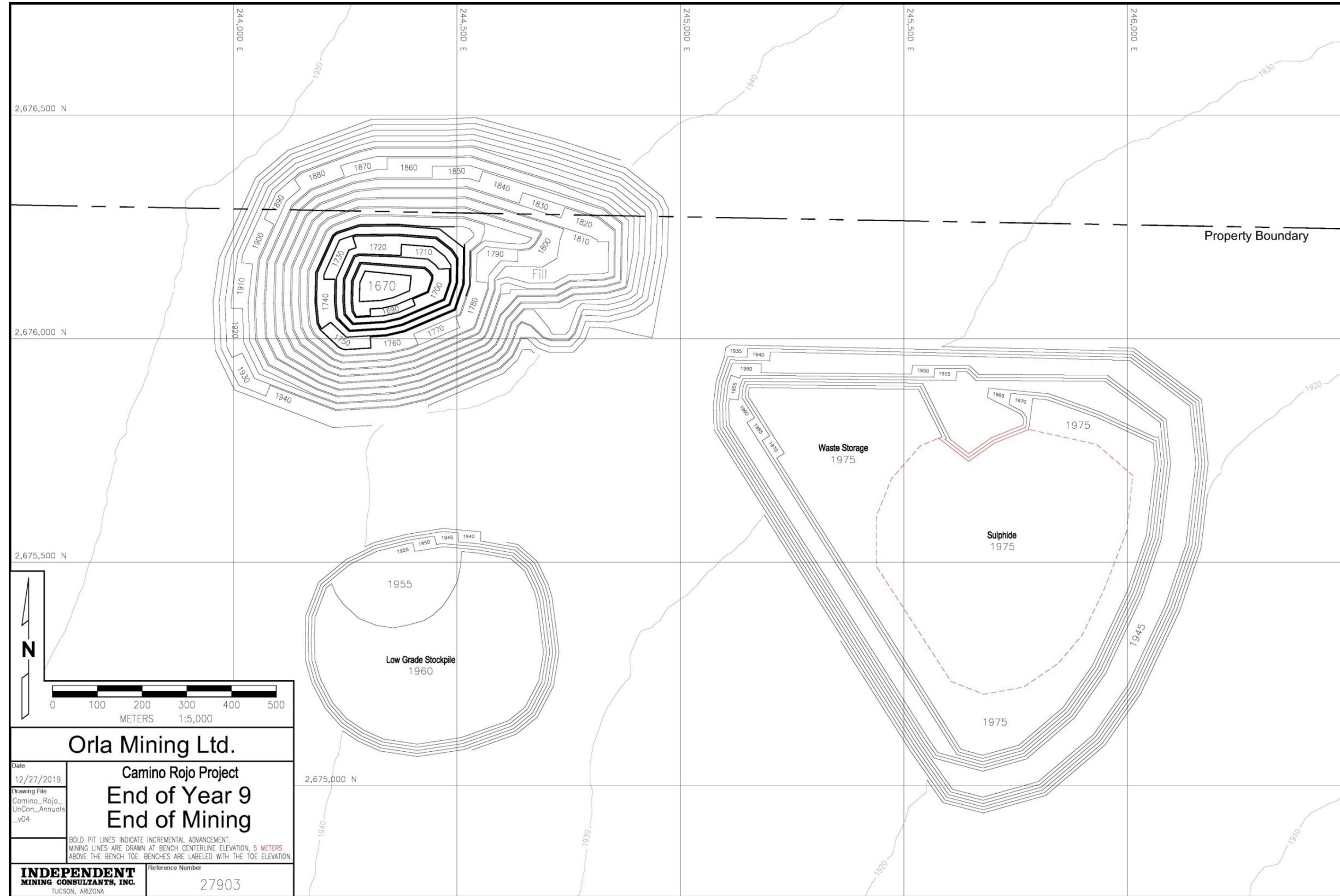
Figure 16.14 Year 9 – End of Mining, IMC 2019
