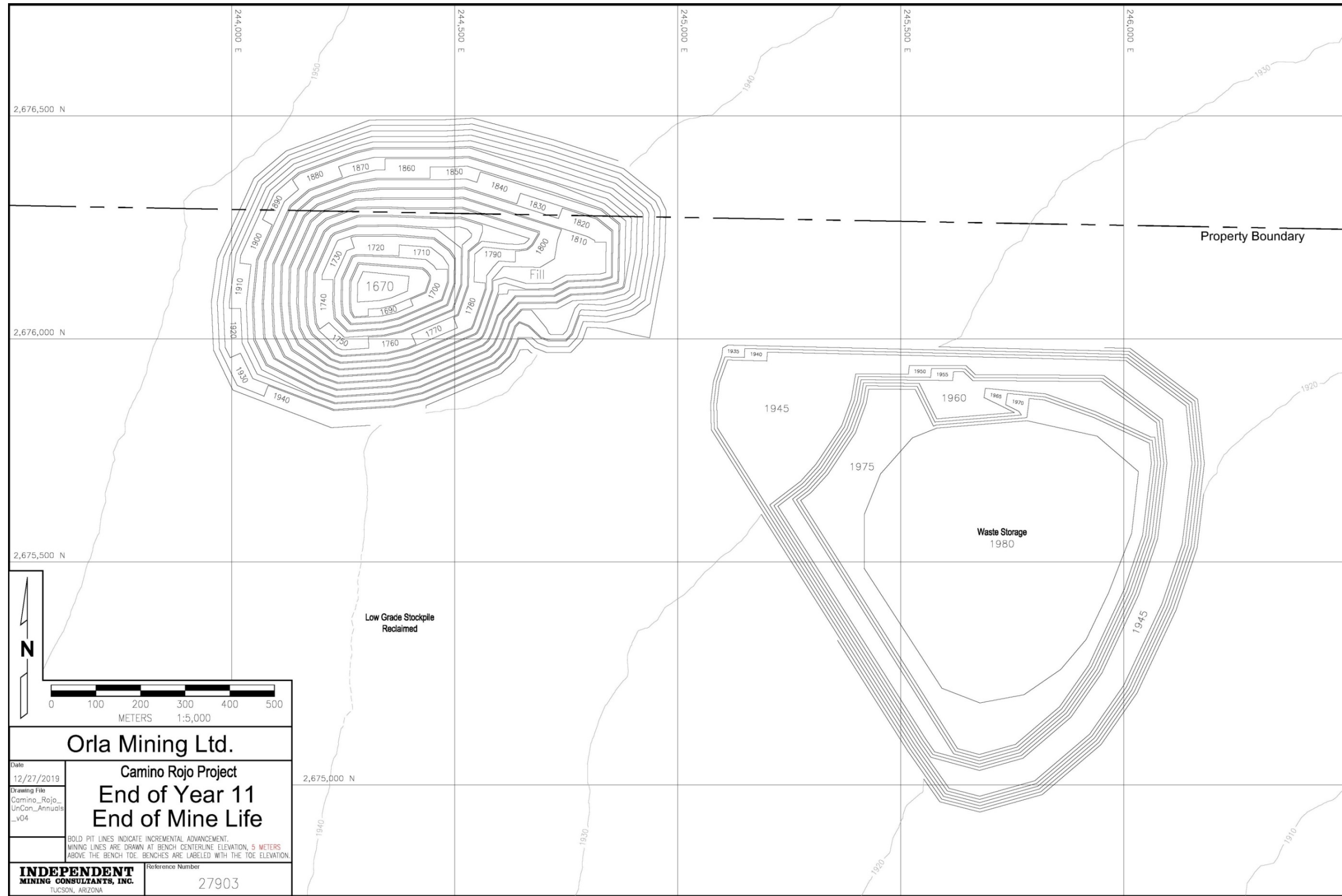
Figure 16.16 Year 11 – End of Low Grade Reclaim, IMC 2019
