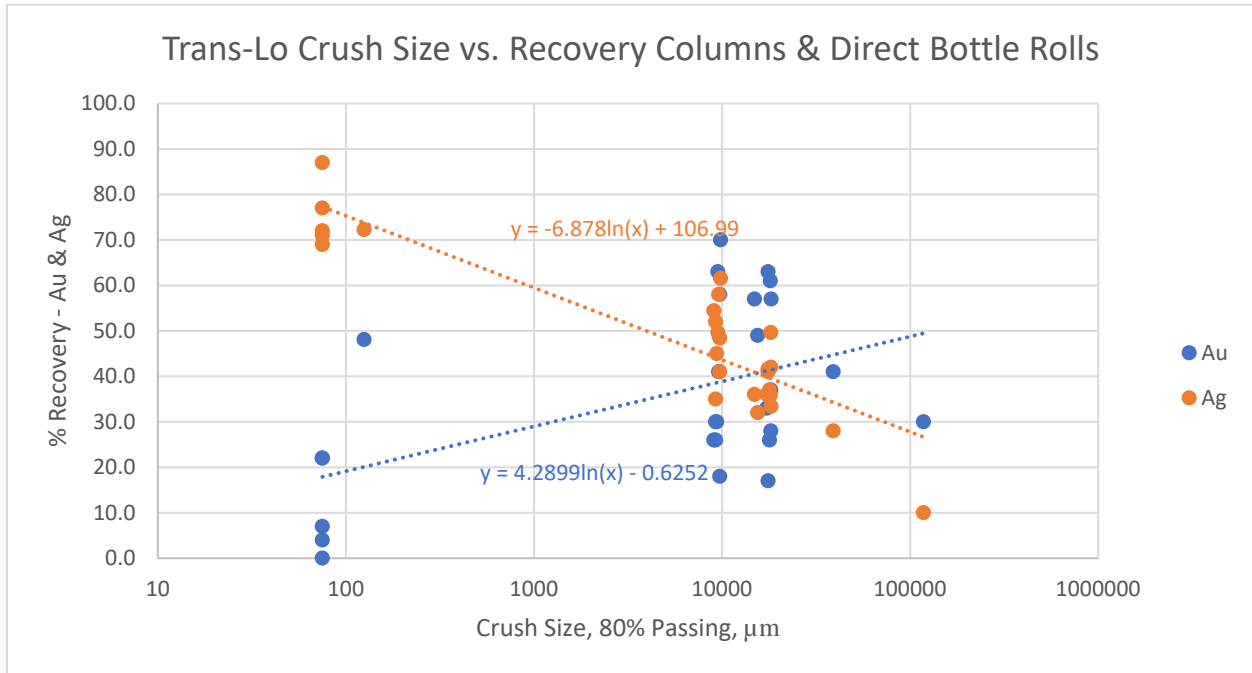
Figure 13.12 Trans-Lo Recovery vs. Crush Size
