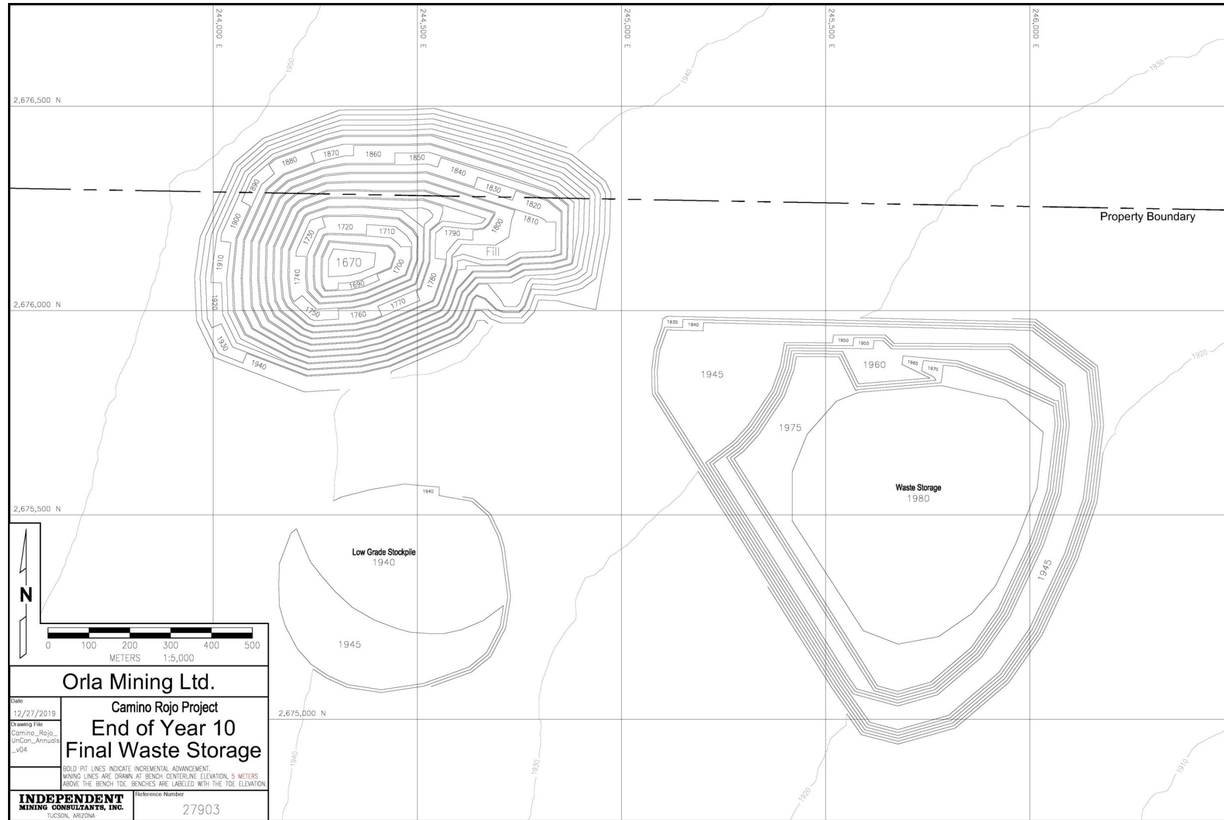
Figure 16.15 Year 10 – End of Waste Storage Capping, IMC 2019
