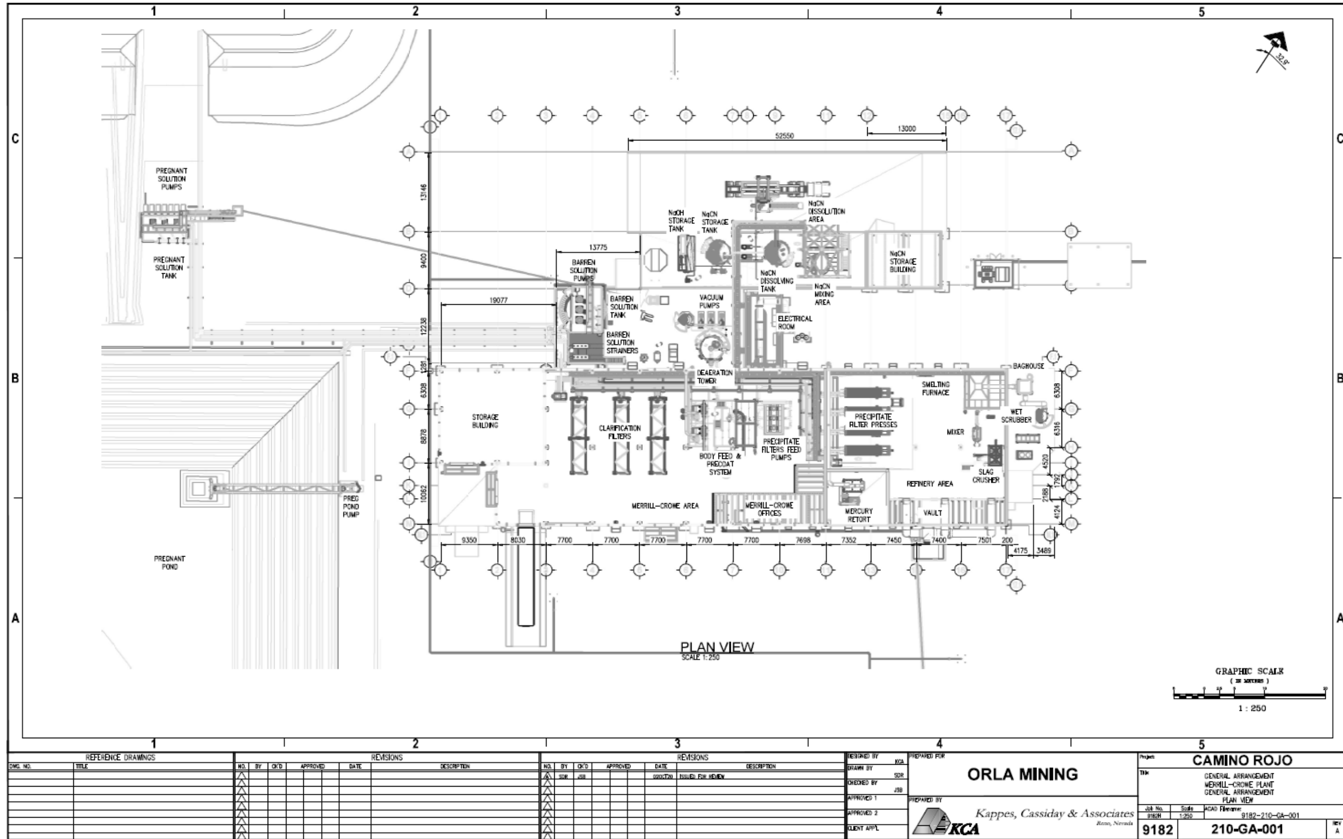
Figure 17.6 Merrill-Crowe Recovery Plant & Refinery Layout
