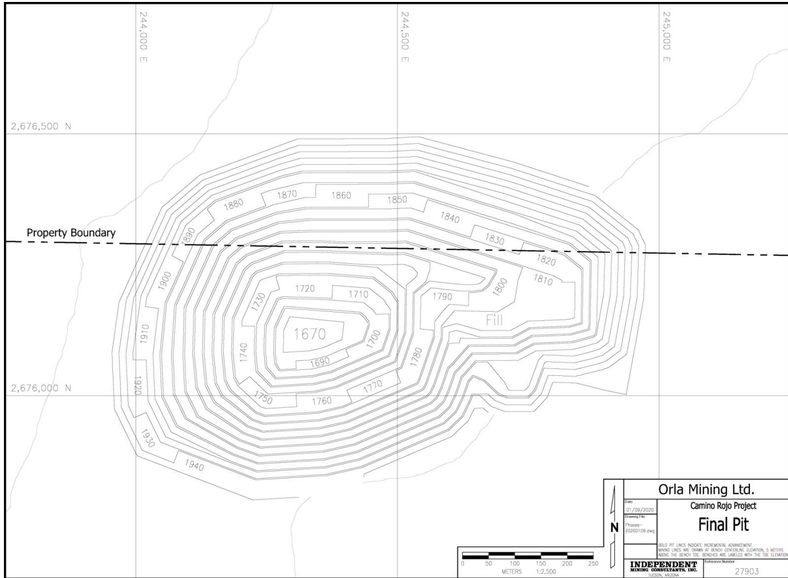
Figure 16.2 Final Pit, IMC 2019
