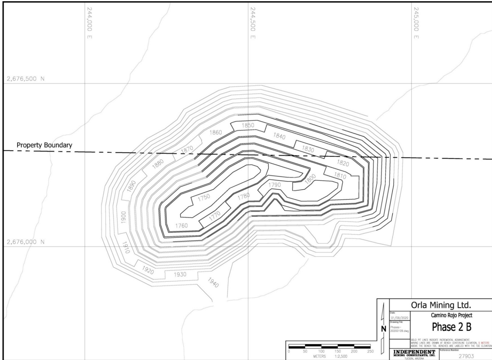
Figure 16.4 Mining Phase 2, IMC 2019
