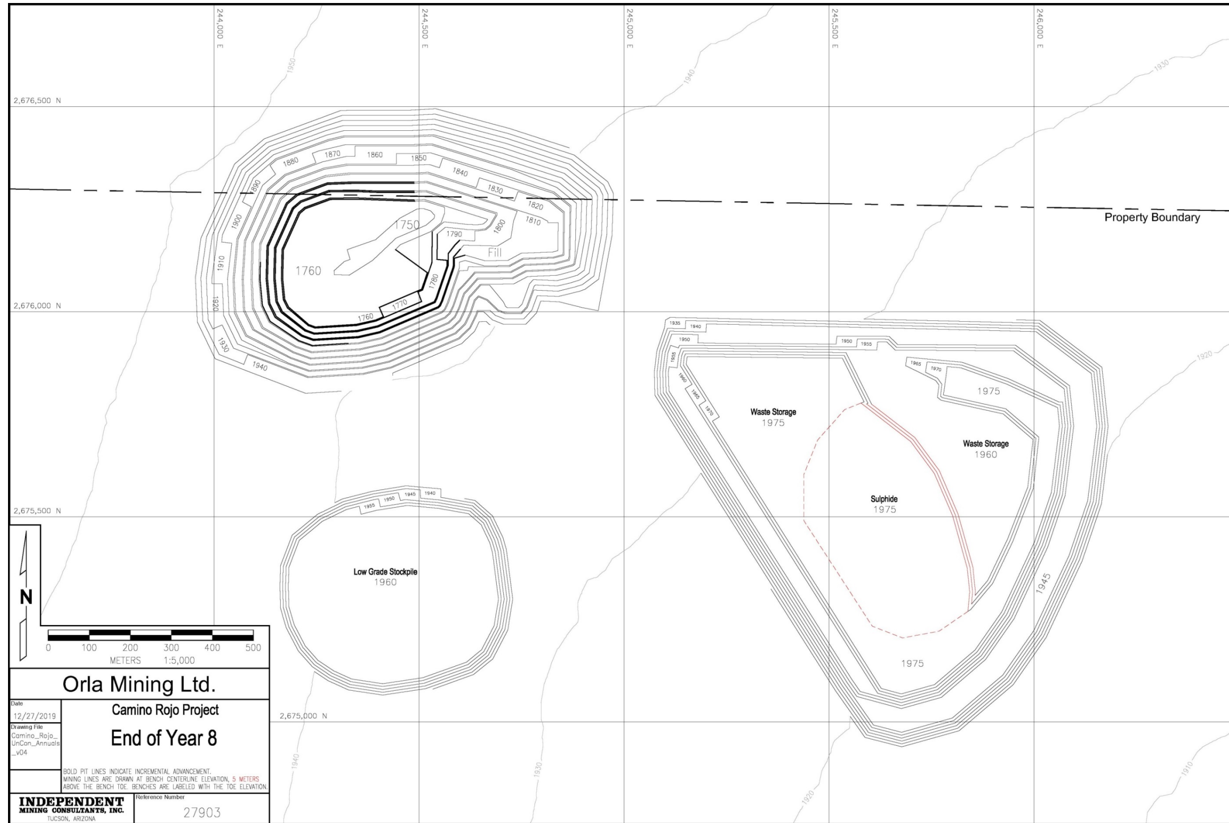
Figure 16.13 End of Year 8 2019
