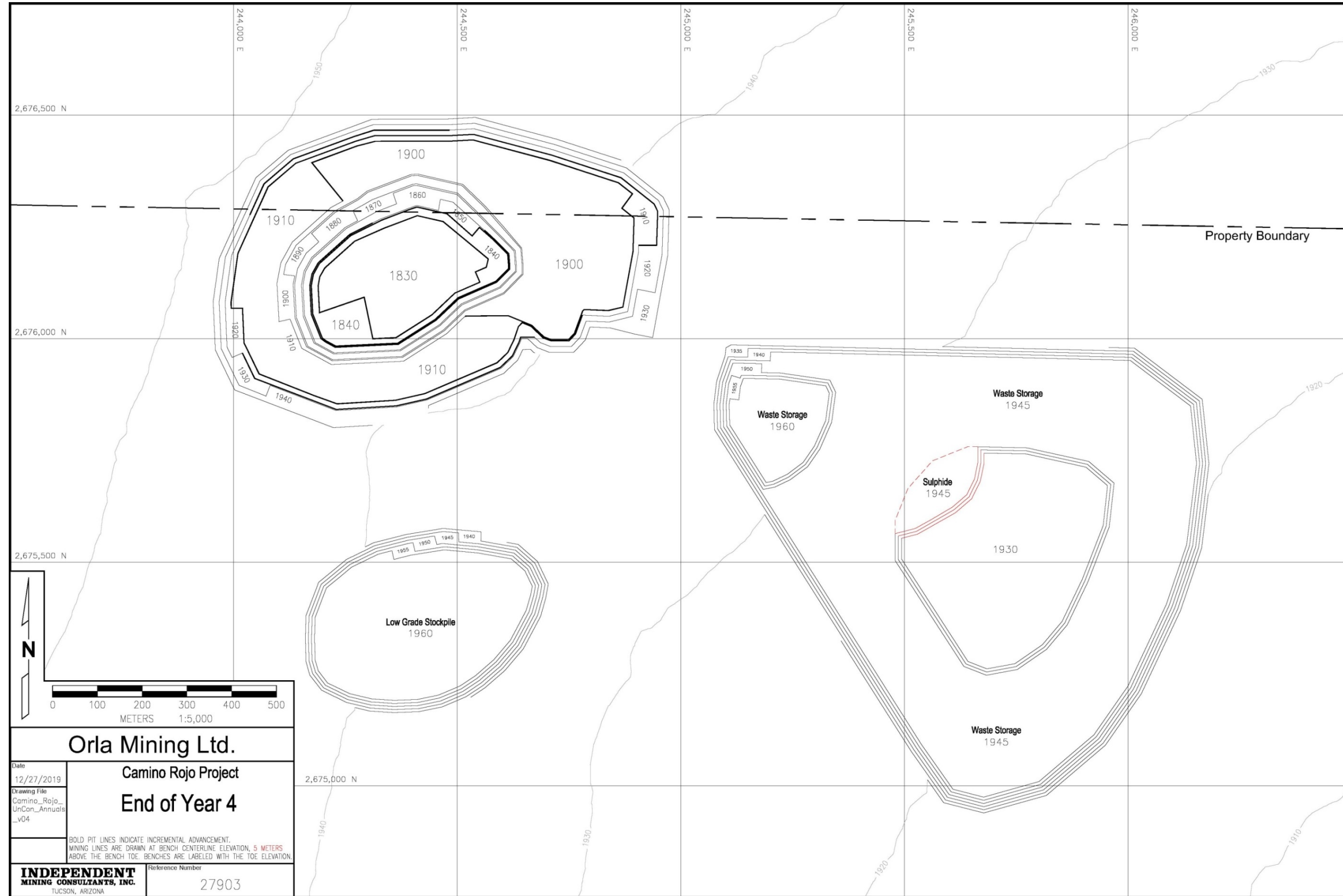
Figure 16.9 End of Year 4, IMC 2019
