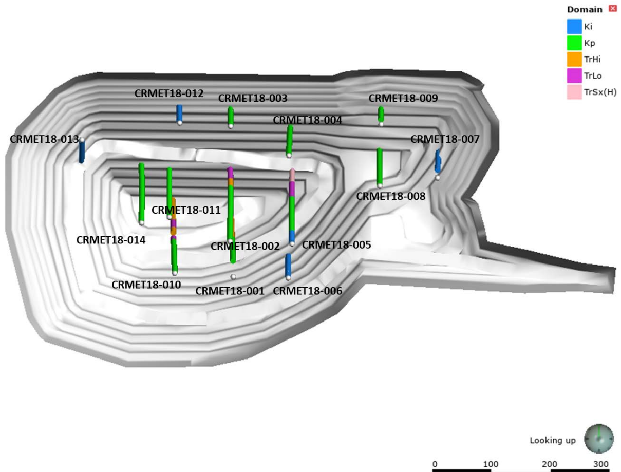
Figure 13.5 Sample Drillhole Locations for KCA 2019 Test Program
