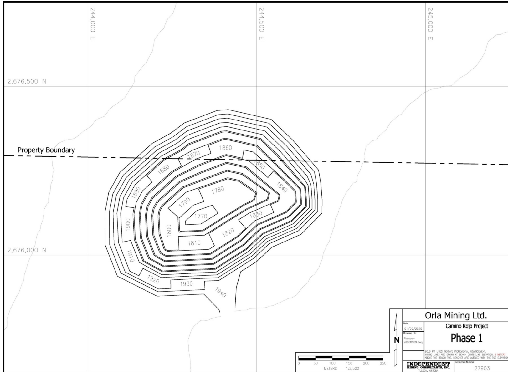
Figure 16.3 Mining Phase 1, IMC 2019
