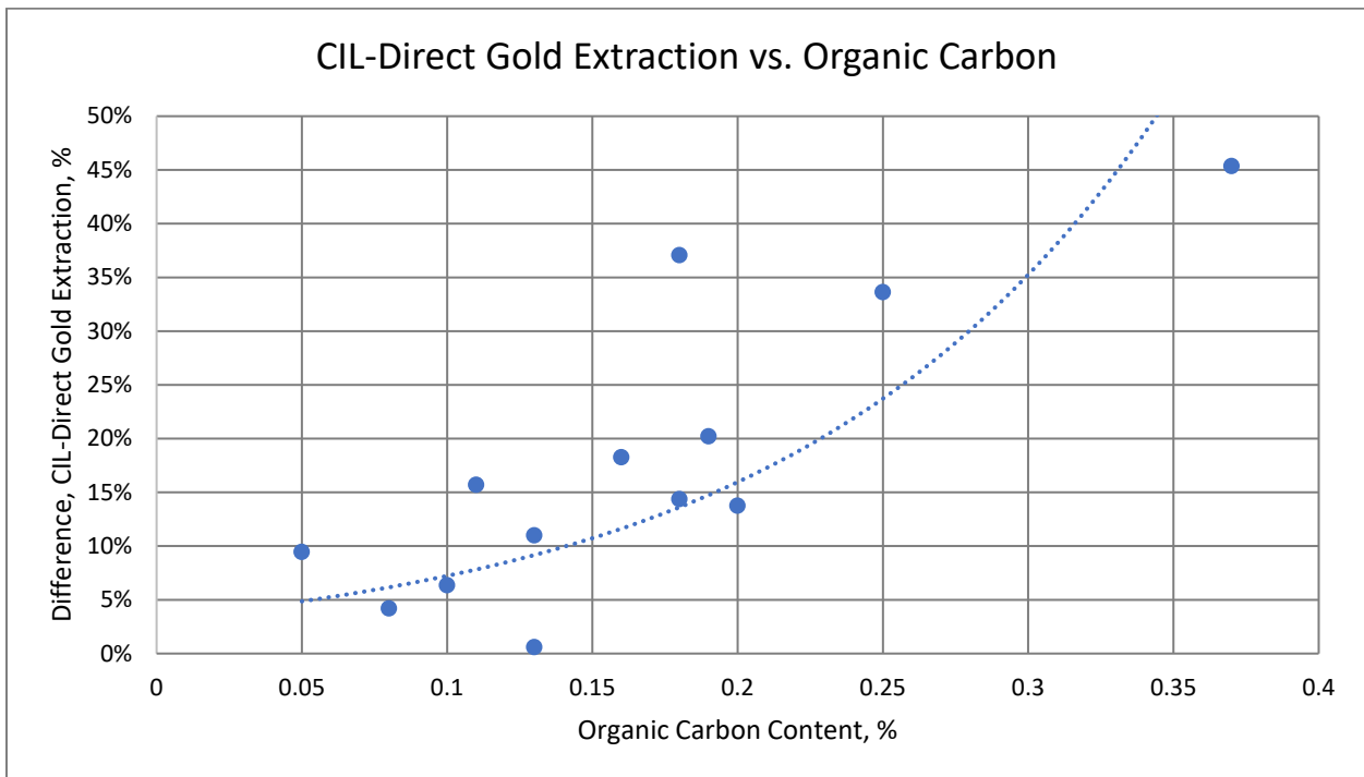
Figure 13.4 CIL-Direct Bottle Roll Au Extraction Difference vs. Organic Carbon Content – KCA 2015
