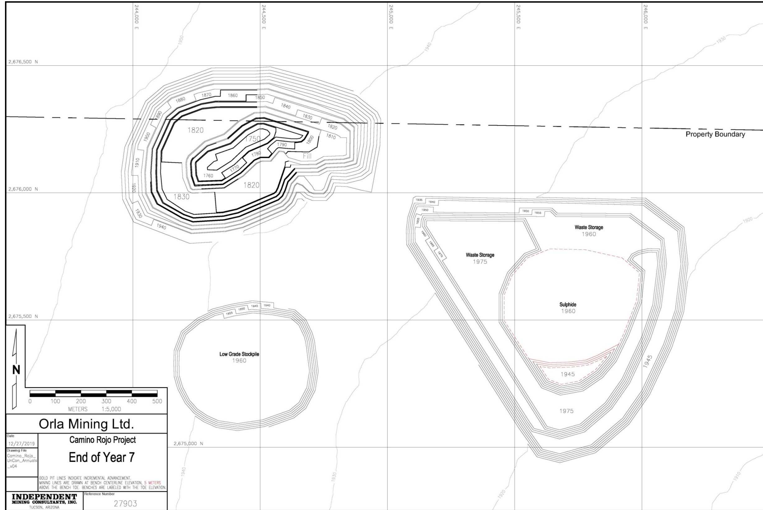
Figure 16.12 End of Year 7, IMC 2019
